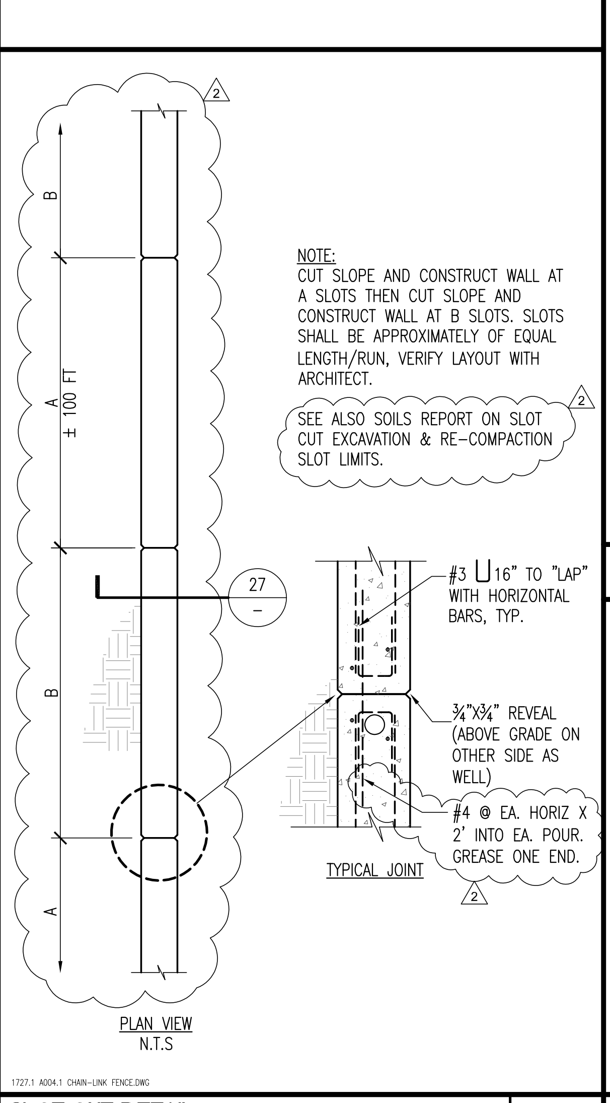
SLOT CUT DETAIL 15 3/4"x1'-0"
