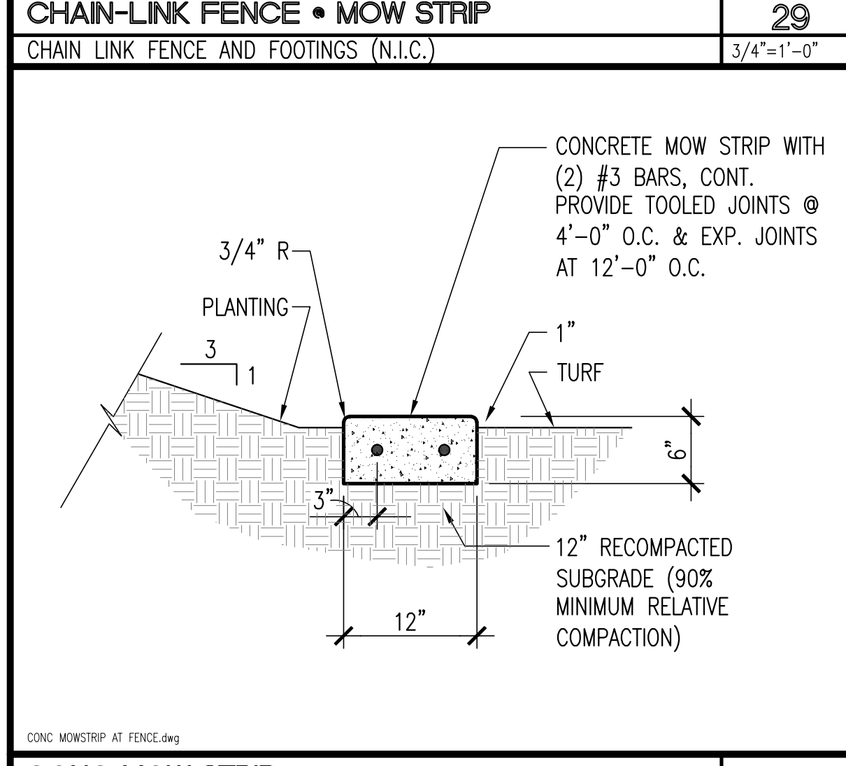
CHAIN LINK FENCE • MOW STRIP 29 CHAIN LINK FENCE AND FOOTINGS (N.I.C.) 3/4"x1'-0"
