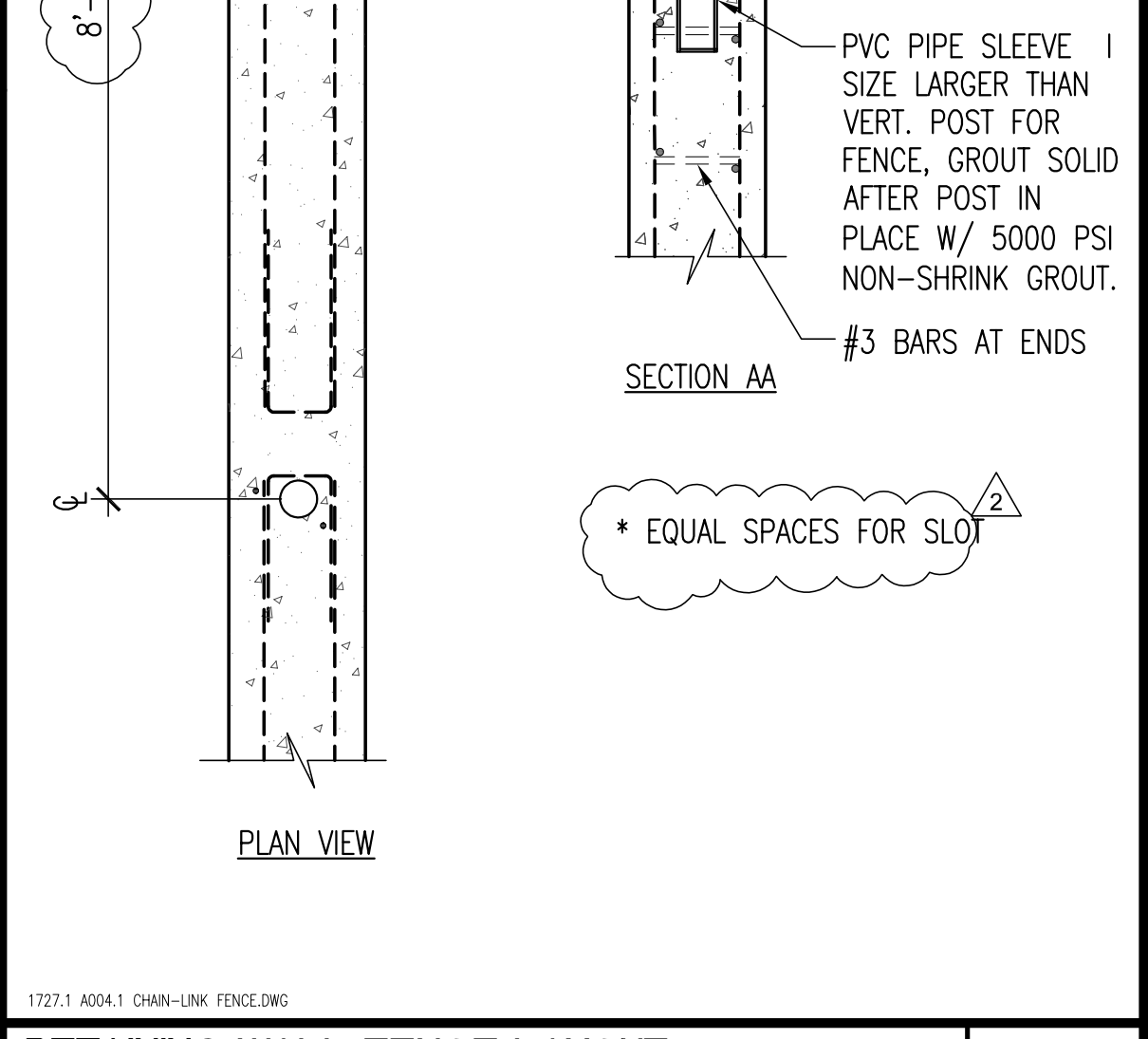
RETAINING WALL FENCE LAYOUT 20 3/4"x1'-0"
