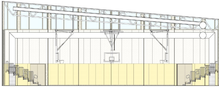
ELEVATION - NORTH
