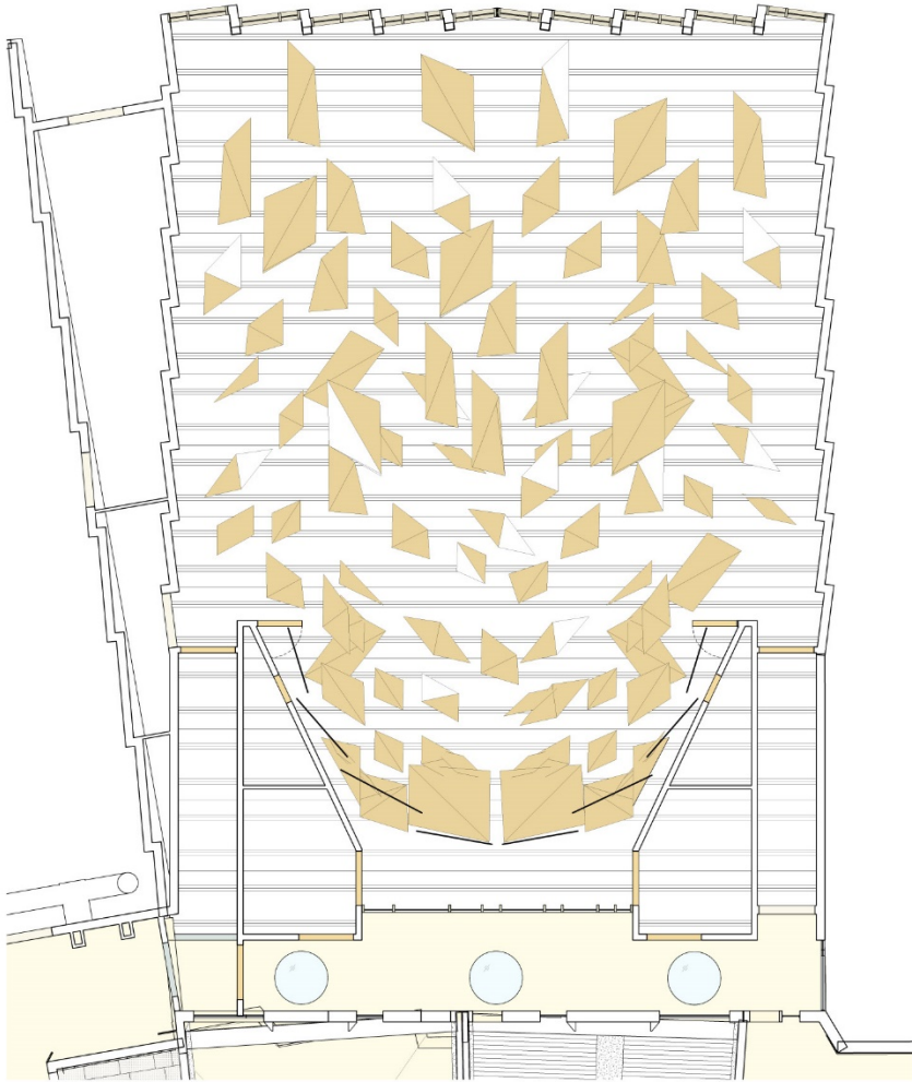
CEILING PLAN
