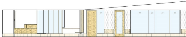
GENERAL ADMINISTRATION_INTERIOR ELEVATION - E
