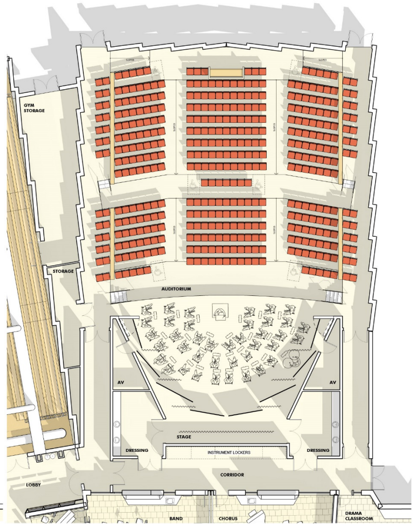
FLOOR PLAN
