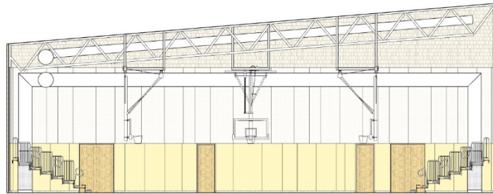
ELEVATION - SOUTH
