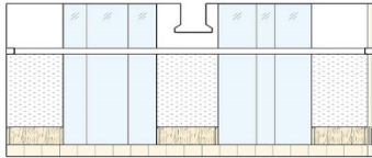
SPED SUITE ELEVATION - S
