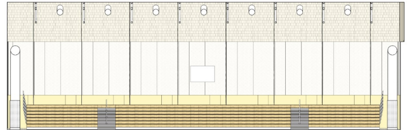
ELEVATION - WEST
