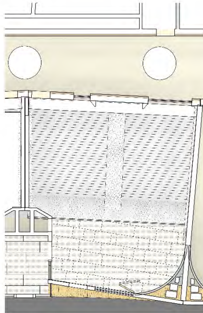
CHORUS ROOM RCP
