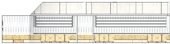
MAKERSPACE ELEVATION - E
