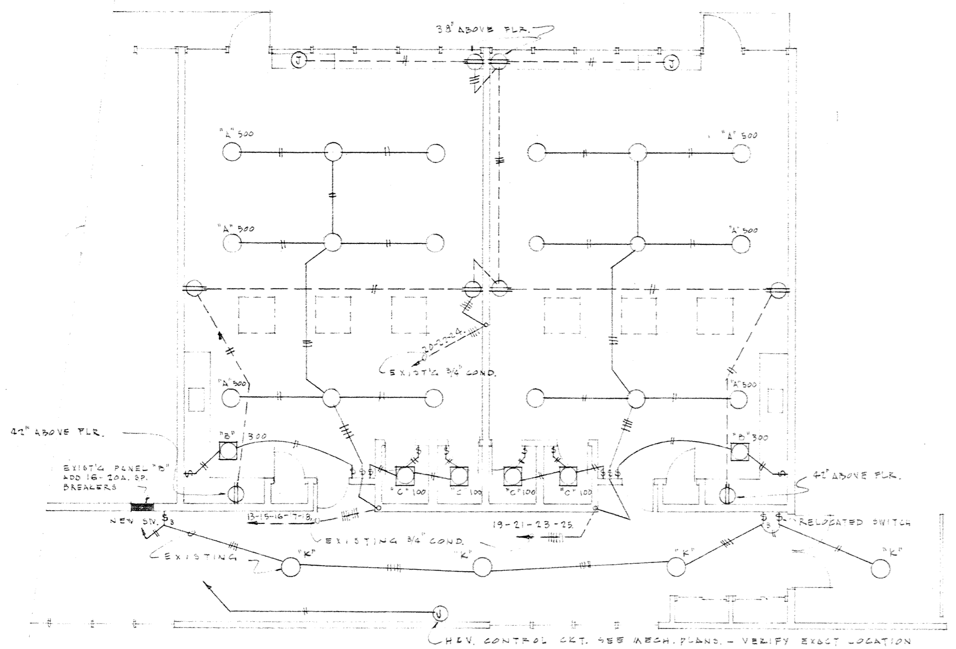
LIGHTING PLAN
