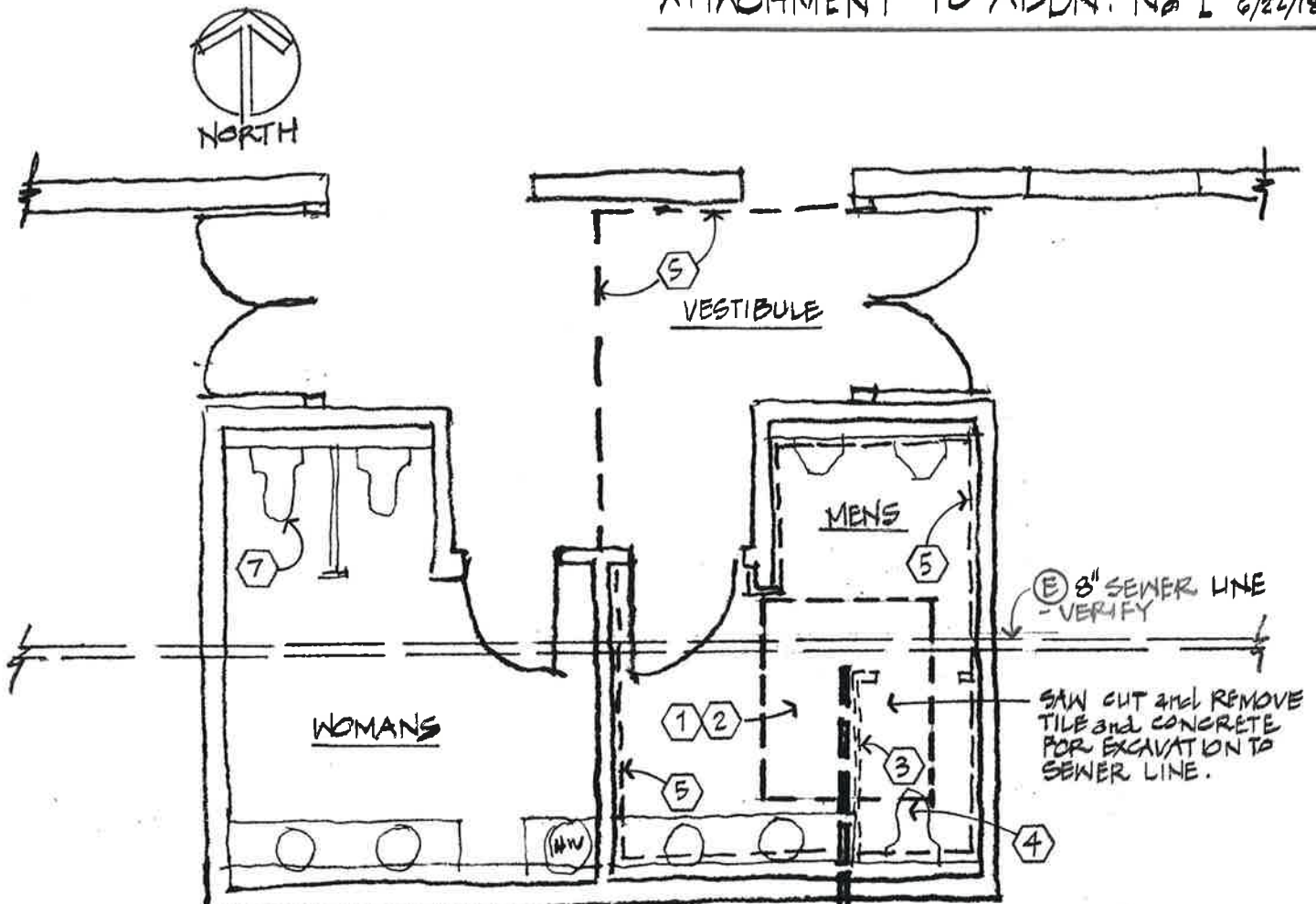
1 PARTIAL PLAN of TRANSPORTATION AD-1 OFFICE TOILET ROOMS no scale
