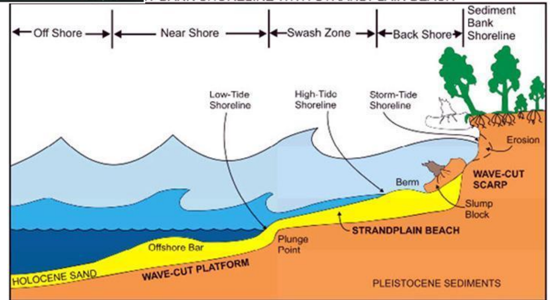
IT-BANK SHORELINE WITH STRANDPLAIN BEACH
