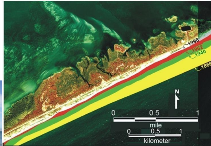
IT-BANK SHORELINE WITH STRANDPLAIN BEACH
