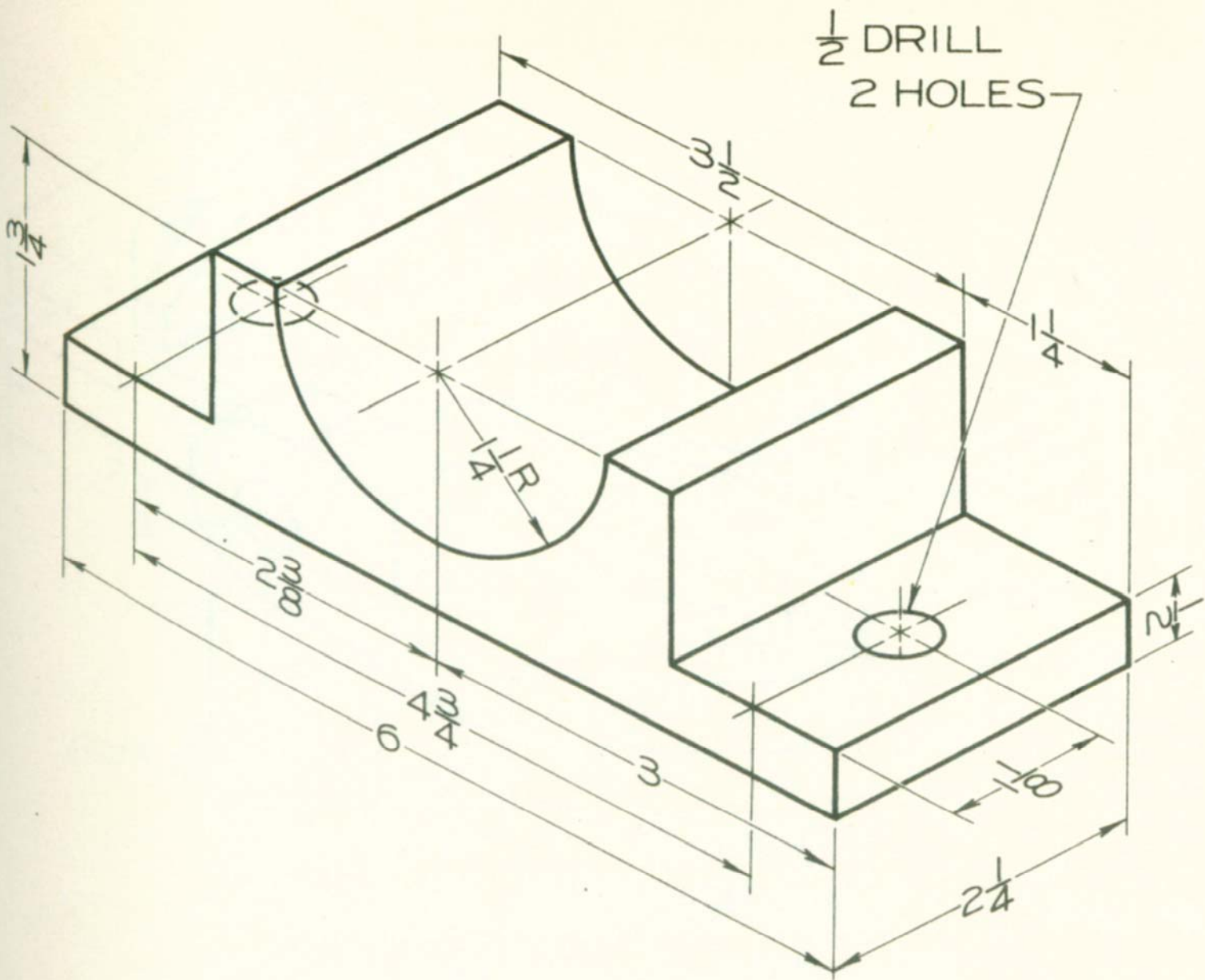
Fig. 257. Trunion Block.*
